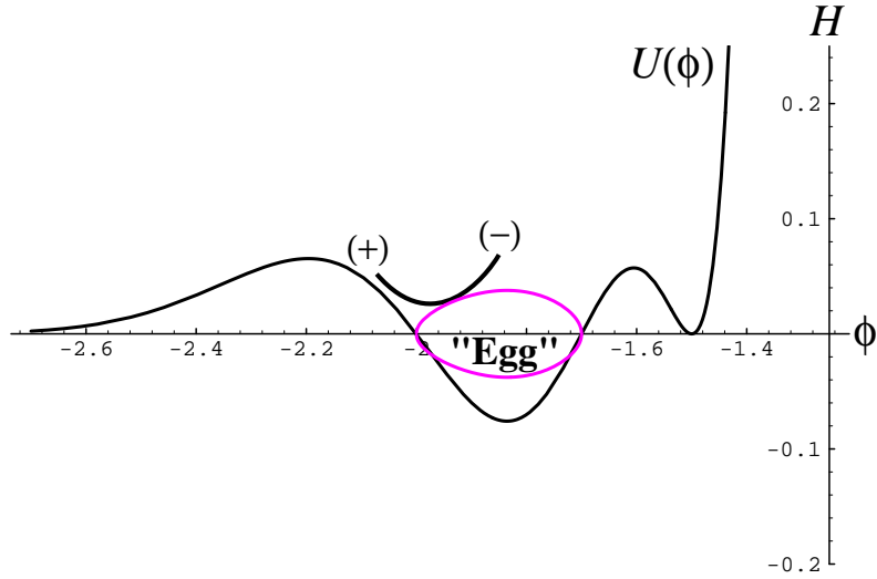
Figure 2. The dilaton potential and corresponding “Egg”. A branch change induced by negative potential.
